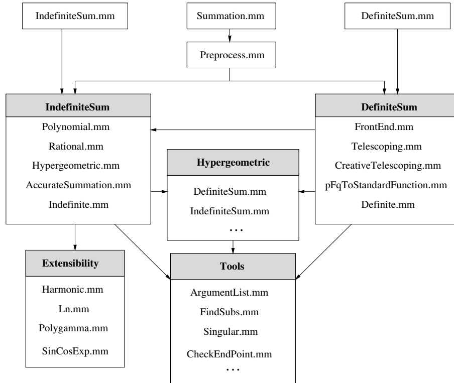
Fig. 5. SumTools package: code structure and code dependency
