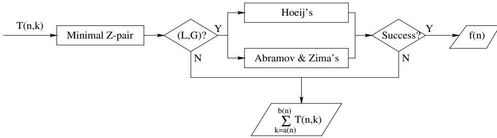
Fig. 3. Definite sums of hypergeometric terms
