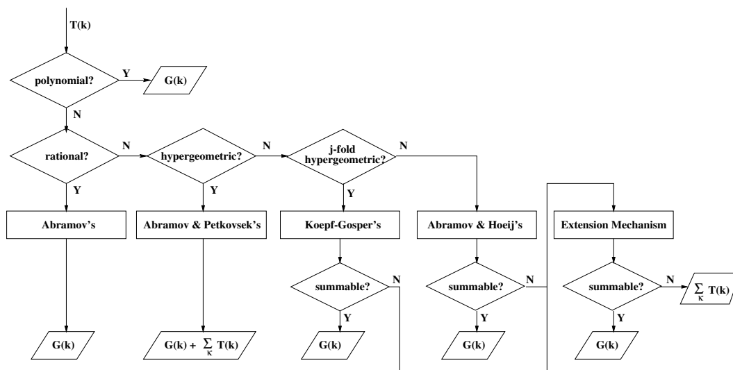
Fig. 1. Indefinite sum: a flowchart
