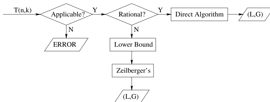
Fig. 2. Algorithms for computing minimal Z -pairs
